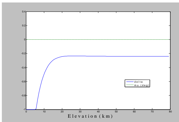
Fig.6 Optimal Controls
