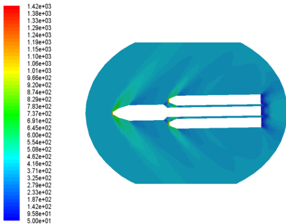
Fig. 4: Pressure contour around the Titan-IV launch vehicle
