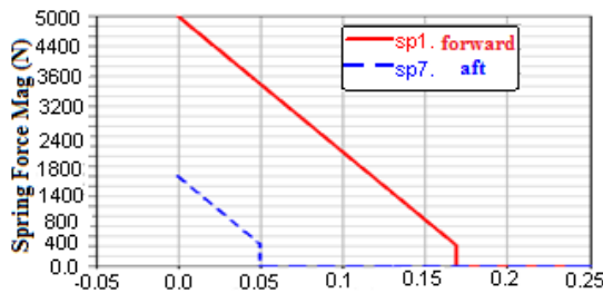
Fig.7: spring ejectors force, as a function of displacement
