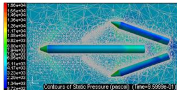
Fig. 2: A view of gridded domain (Dynamic Mesh Updating)
