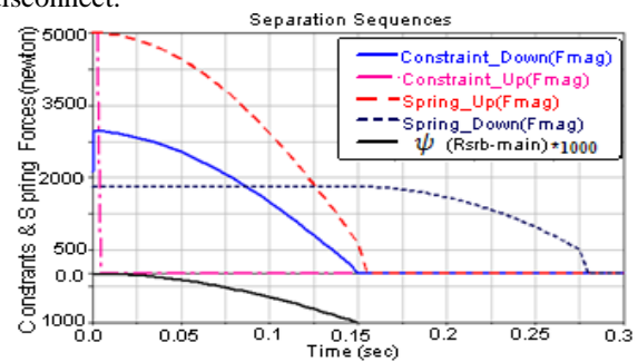
Fig. 9: Separation sequence of spring ejectors and joints
