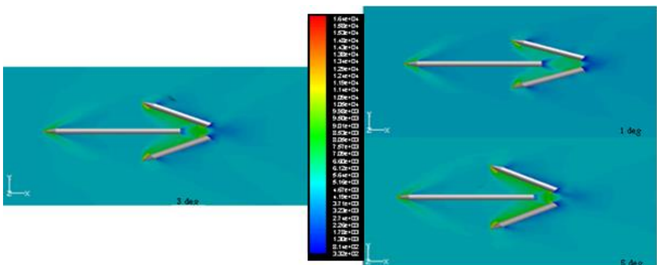
Fig. 24: Pressure contour variation around the launch vehicle and boosters at t=1.1 sec after separation (with various separation angle conditions - using standard ejector springs) CM) with time with various separation angle conditions (in the presence of aerodynamic effects)
