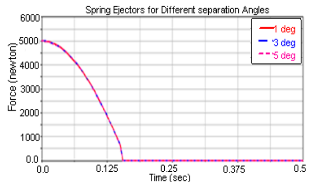
Fig. 23: Time variation of spring force for various separation angle conditions
