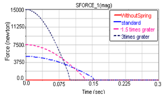
Fig. 14: Time variation of spring force for spring ejectors with different powers
