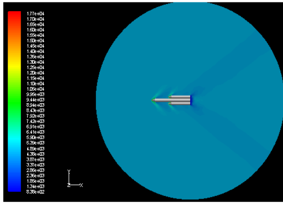
Fig. 3: flow field around the launch vehicle
