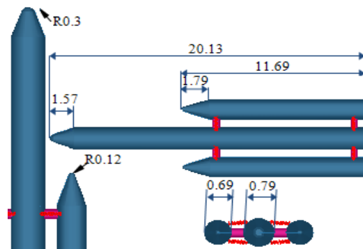
Fig .1: launch vehicle configuration (meter)
