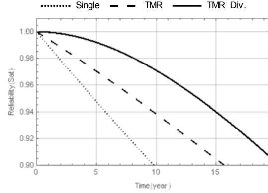
Fig. 9: Reliability of a TMR system (satellite case) with and without HW/SW diversity versus time.
