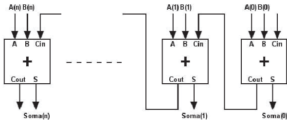
Fig.11 Block diagram of a ripple carry adder
